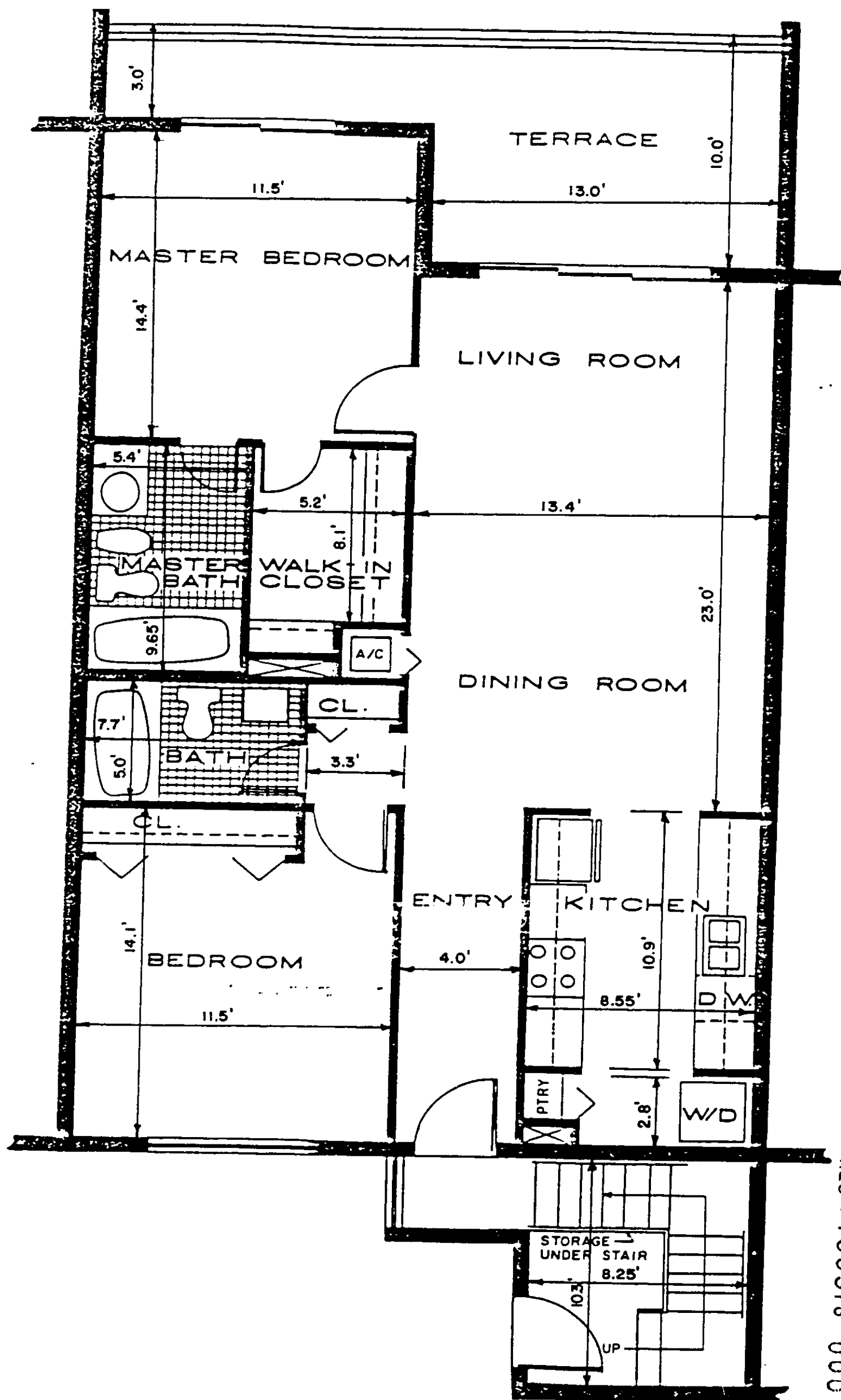
UNIT TYPE "C" FLOOR PLAN
