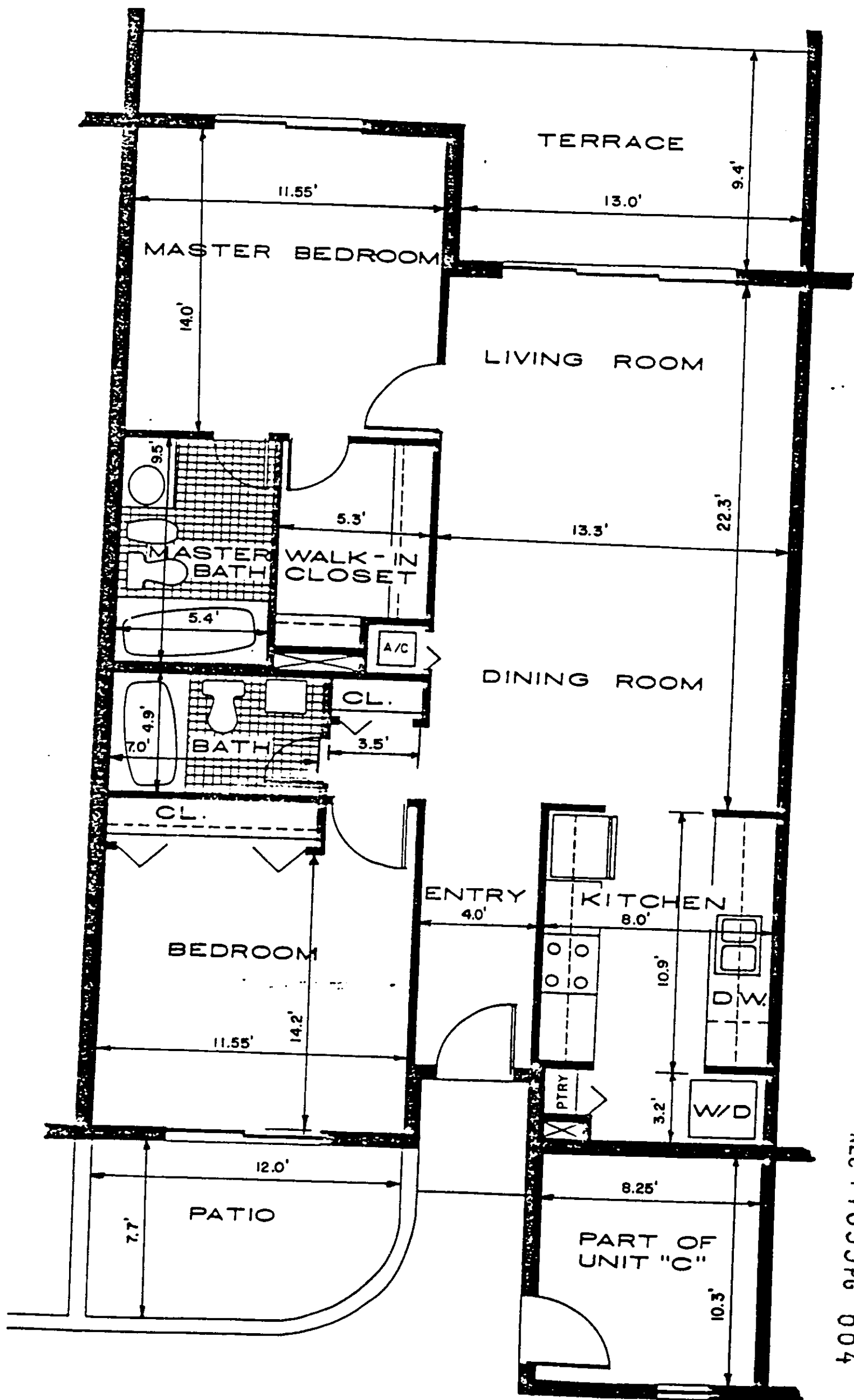
UNIT TYPE "B" FLOOR PLAN
