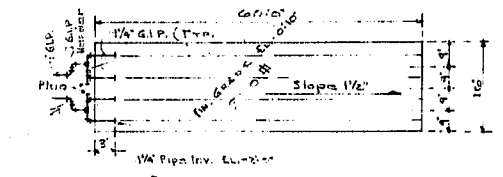
PLAN OF DRAINFIELD Scale: 1/8" = 1'-0"
